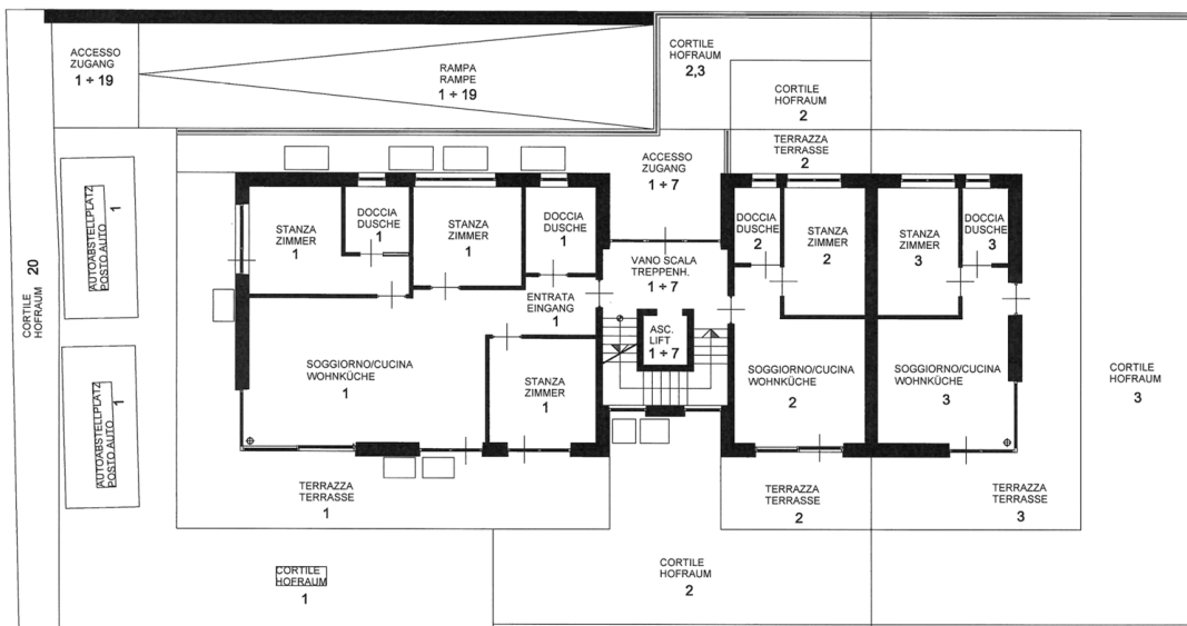
ERDGESCHOSS PIANO TERRA
